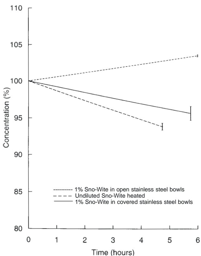
Fig 5. Change in percentage concentration with time of available chlorine of undiluted Sno-Wite heated to 50°C and diluted Sno-Wite stored in open and closed stainless steel bowls for periods up to six hours.
