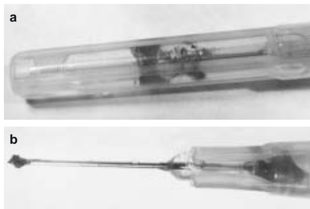
Fig 4. Rust formation after seven days in syringes loaded with Milton and stored in the dark. Fig 4a shows demonstrable rust formation in drops of Milton trapped in needle sheath of syringe. In Fig 4b, the lumen of the 30 gauge needle appears completely occluded by rust.
