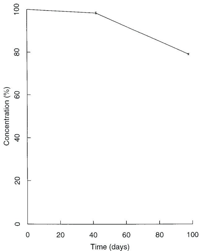
Fig 3. Change in percentage concentration with time of available chlorine in Sno-Wite diluted to 1 per cent when stored in translucent syringes stored in the dark.
