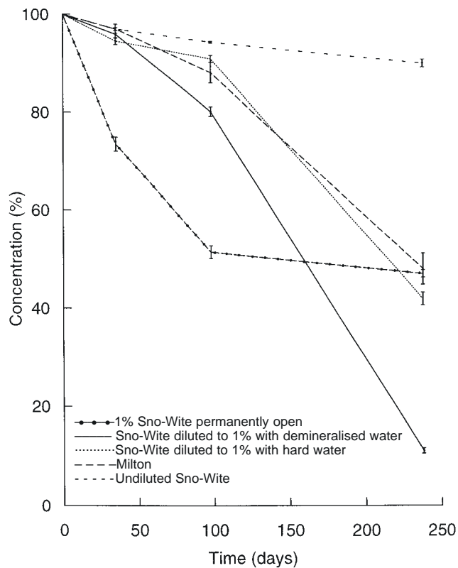
Fig 1. Change in percentage concentration of available chlorine in sodium hypochlorite solutions stored over eight months while opened and agitated daily or left permanently open.
